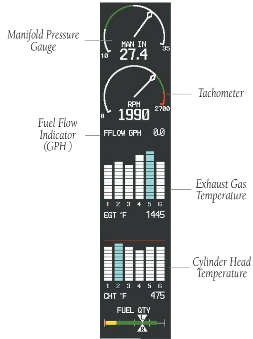
Figure 3-2 LEAN Page (182T Shown)
