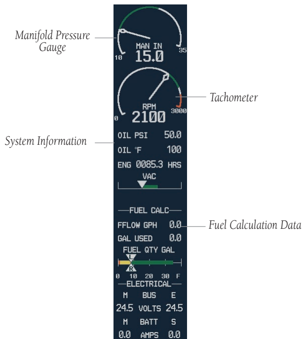
Figure 3-3 Engine System Window (206H Shown)
