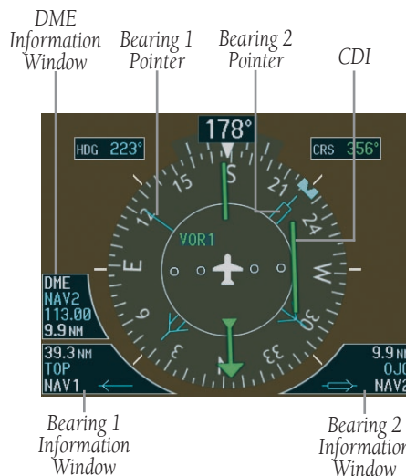
Figure 2-14 HSI with Bearing Information
