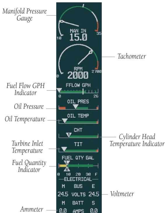
Figure 3-1 Engine Indication Window (T182T Shown)
